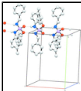
Fig. 2. Part of the crystal packing of the title compound with the hydrogen bonds shown as dotted lines (the C—H hydrogen atoms are omitted for clarity).
